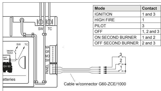
Figure 1: Wiring diagram and the operation sequence
